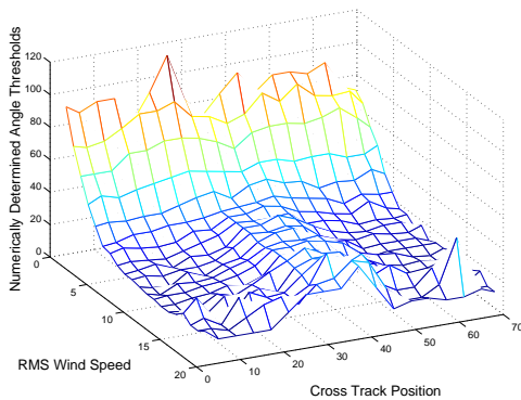
Figure 8: The direction thresholds per cross track and rms wind speed that minimize the probability of false alarm beneath a threshold of 2.5%.
