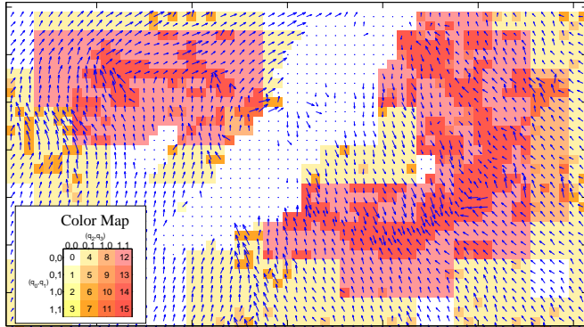
Figure 15: QA bit flag example containing a possible region of ambiguity selection error. Missing vectors indicate the position of land. Notice that the QA algorithm flags the position of inconsistencies in the estimated wind flow.
