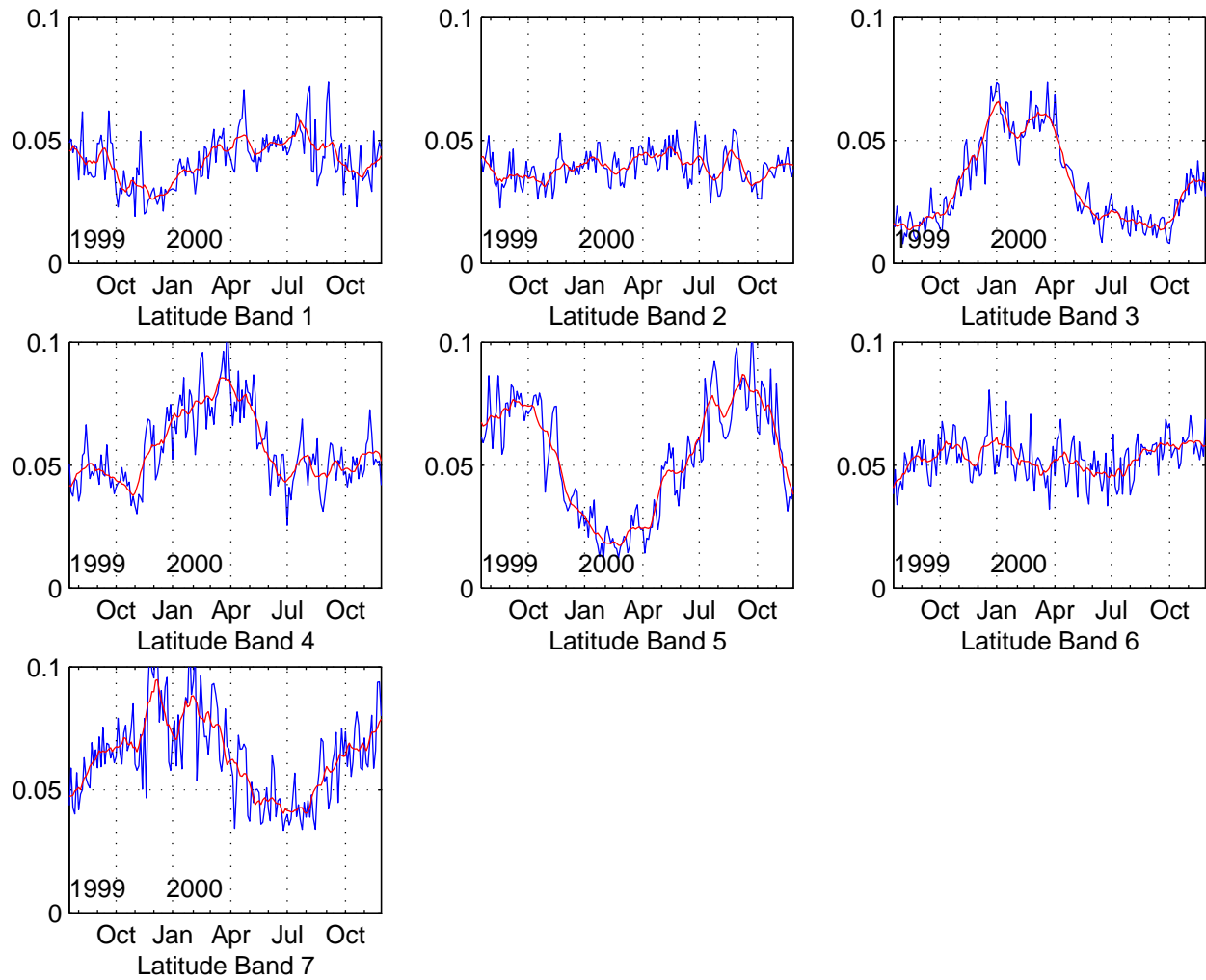
Figure 23: Fraction of ambiguity selection errors averaged over three days (blue) and moving averaged over 30 days (red) for each latitude band.
