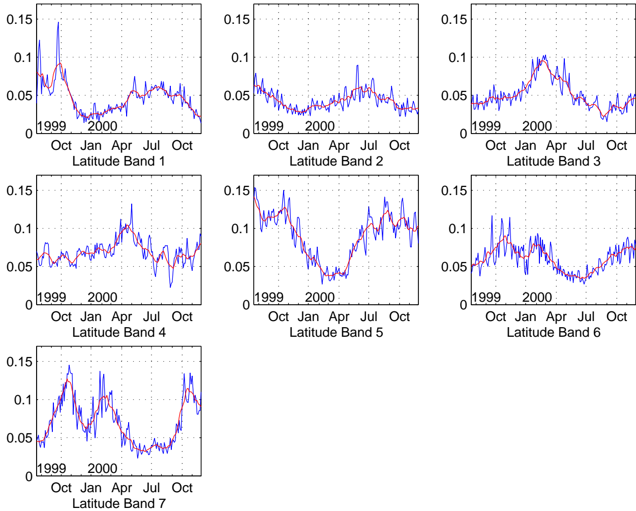
Figure 22: Fraction of cells flagged as containing rain averaged over three days (blue) and moving averaged over 30 days (red) for each latitude band.
