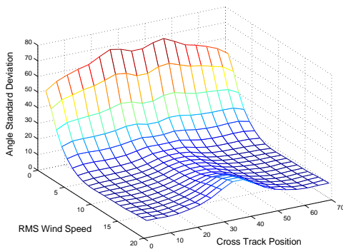
Figure 7: The average directional standard deviation for both rms wind speed and cross track position.
