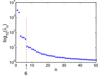
Figure 1: The first 50 eigenvalues of the 8 \times 8 KL model.
